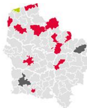
particules PM2.5
