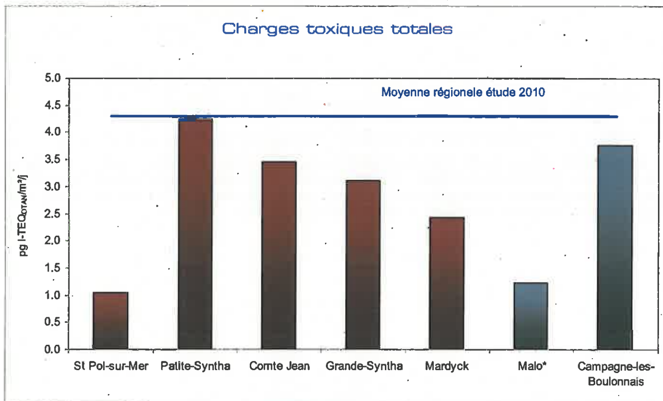
Figure 25: Charge toxiqua globala exprimée an pg I-TEQ OMS /m 2 /j
